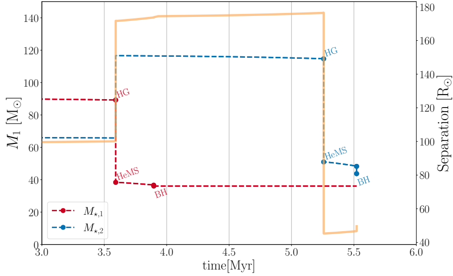
Figure 3.10: Masses (dashed lines, left y-axis) and binary orbital separation (solid yellow line, right y-axis) over time, for a typical BBH progenitor system that evolved through the stable RLOF channel. Transitions to different evolutionary stages are labelled with the following acronyms: HG for Hertzsprung Gap star, HeMS for He Main Sequence star and BH for Black Hole.
