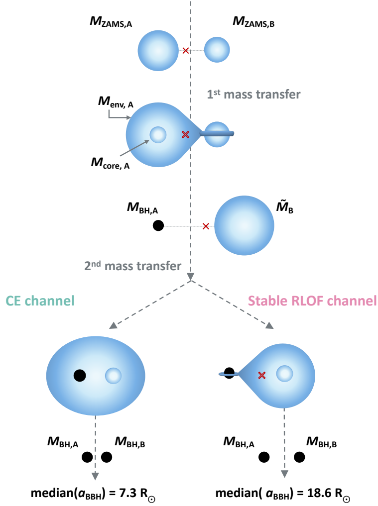
Figure 3.1: Cartoon depiction of the typical evolution of a BBH progenitor system through the stable RLOF and CE channel. Annotations refer to masses at zero age main sequence ( M_{\text{ZAMS}} ), the envelope mass ( M_{\text{env}} ), the core mass ( M_{\text{core}} ), mass post mass transfer ( \tilde{M}_B ) and BH mass ( M_{\text{BH}} ). The subscript A (B) denotes the initially more (less) massive star. The red cross gives an impression of the location of the centre of mass at the onset of the evolutionary phase depicted (not to scale). The median separation at BBH formation is annotated for each channel, considering BBH mergers that can be observed by a ‘perfect detector’ (see text).
