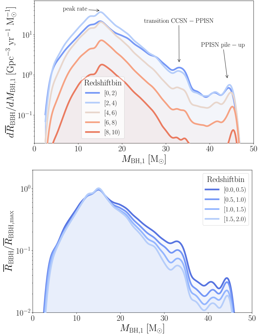
Figure 3.6: Distribution of primary BH masses M_{\text{BH},1} for several redshift bins. The top panel shows the general trend for different redshift bins. The bottom panel shows the same distribution normalized by the peak rate value for the given redshift bin, with a focus on redshifts up to z = 2 . Both distributions are shown down to M_{\text{BH},1} = 2.5 M_{\odot} , which is our minimum allowed BH mass. This shows that the distribution of primary BH masses evolves with redshift.
