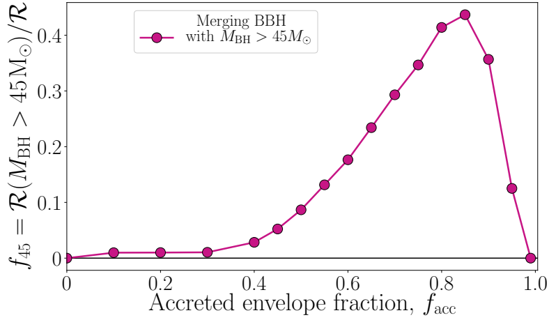
Figure 2.7: The fraction of BBH mergers with a component mass M_{\text{BH}} > 45 M_{\odot} (i.e. f_{45} ), as a function of the fraction of the companion’s envelope that is accreted during each CE mass transfer episode. Each point represents one simulation from the additional exploratory grid of 17 simulations discussed in Section 2.6.1.
