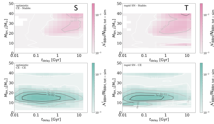
Figure 3.16: Same as Figure 3.14 but for the following model variations: Panel S: Hertzsprung-gap donor stars initiating a CE are allowed to survive this CE event. Panel T: adopts the Fryer et al. (2012) “rapid” supernova remnant-mass prescription.
