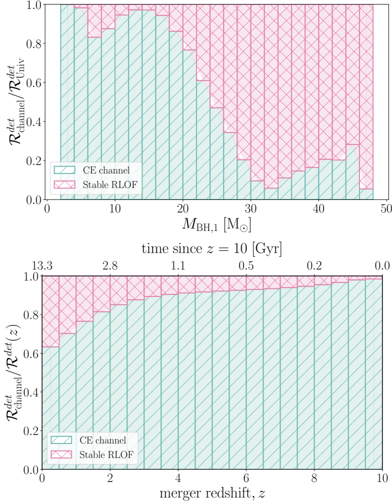
Figure 3.4: Fractional contribution of the CE channel (green hatched) and the stable RLOF channel (pink cross hatched) to \mathcal{R}^{\text{det}}(z, \zeta) . Top panel shows the relative contributions to \mathcal{R}^{\text{det}}(z, \zeta) per mass bin after integrating over all redshifts. Bottom panel shows the fractional contribution to \mathcal{R}^{\text{det}}(z, \zeta) integrated over all M_{\text{BH},1} , as a function of redshift.
