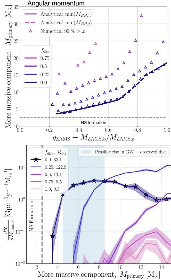
Figure 5.5: Same as Figure 5.3, but for variations in the fraction of the mass that is assumed to be lost from a circumbinary disk, f_{\text{disk}} . Because Equation 5.10 does not capture variations in the orbital angular momentum loss, we only show the analytical solution for f_{\text{disk}} = 0.0 in the top panel. Furthermore, we do not show f_{\text{disk}} = 1.0 in the top panel because it contains too few samples to properly bin the distribution.
