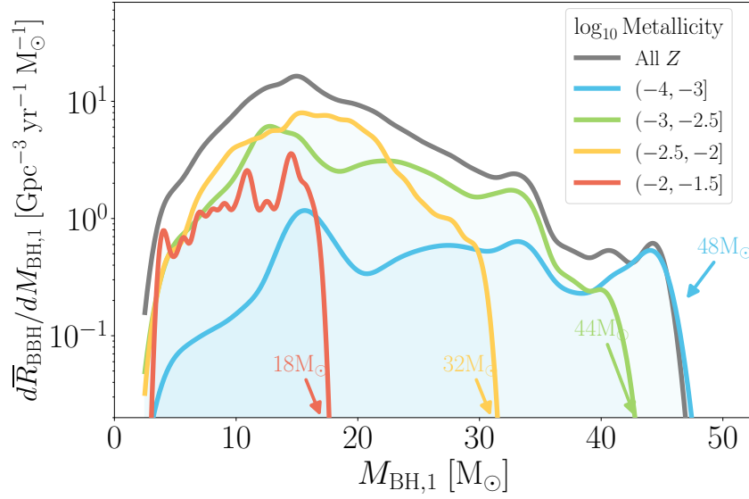
Figure 3.7: Breakdown of the M_{\text{BH},1} mass distribution by birth metallicity for all BBH mergers between redshifts 0 \leq z < 0.5 . The maximum BH mass that contributes to each metallicity bin is annotated.
