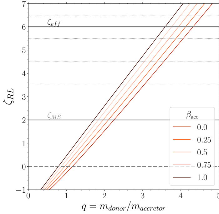
Figure 5.6: \zeta_{\text{RL}} as a function of mass ratio of between the donor and accretor star. Mass transfer is dynamically stable as long as \zeta_{\text{RL}} \leq \zeta_{\text{eff}} . The intersections of \zeta_{\text{RL}} and \zeta_{\text{eff}} reveal different values of q_{\text{crit},1} and q_{\text{crit},2} . Our default value of \zeta_{\text{eff}} = 6.0 for a star with a clear core-envelope structure is annotated. \zeta_{\text{MS}} = 2 shows the adopted stability criteria assumed for main-sequence stars (Ge et al., 2015)
