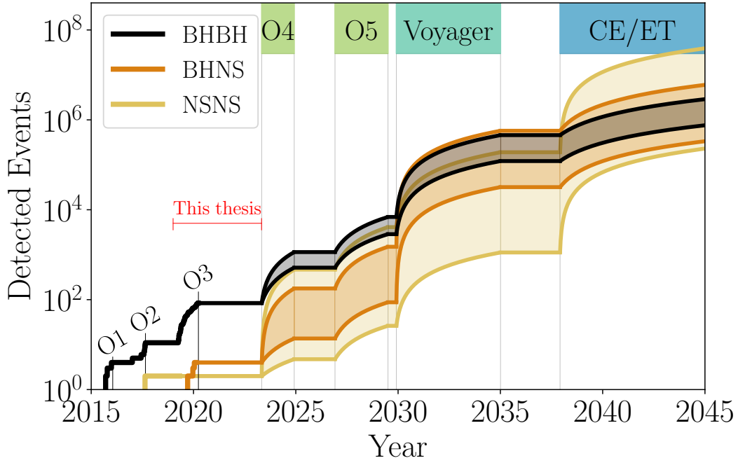
Figure 1.1: The current and projected size of the GW-source catalog. Detection rates and mission times for observing run O4 and O5 are taken from Abbott et al. (2018b) and the ligo doc pages . Detection rates for Voyager, Cosmic explorer (CE) and the Einstein telescope (ET) follow from Borhanian & Sathyaprakash (2022) , and Gupta et al. (2023) . Mission times are only indicative for the latter detectors. The minimum and maximum number were calculated using the redshift-independent rates from Abbott et al. (2021e) .
