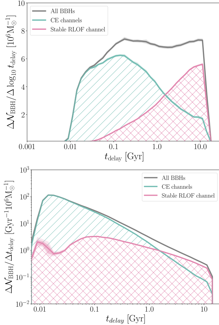
Figure 3.11: Similar to Figure 3.2, but integrated over M_{\text{BH},1} . The solid line shows the centres of the histogram per d \log_{10} t_{\text{delay}} (top panel) versus the histogram per dt_{\text{delay}} (bottom panel), with bin sizes that are equal size in log-space ( d \log_{10} t_{\text{delay}} = 0.1 ), and hence unequal size in t_{\text{delay}} . Both are normalized per 10^6 \text{M}_{\odot} of star forming mass. This histogram contains a mixture of birth metallicities, that were sampled uniformly in log. The dark and light shaded areas shows the 1- and 2- \sigma bootstrapping uncertainties respectively. We indicate the stable RLOF channel with pink cross hatched lines, and the CE channel with green line hatches.
