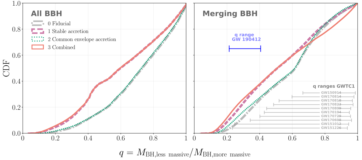
Figure 2.4: Cumulative distribution function of the mass ratio q , defined as the ratio of the less massive over the more massive BH. The left panel shows all BBHs, while the right panels displays only the BBH population that merges within a Hubble time. The 90% confidence interval of observed mass ratios are shown as gray lines for observations from LIGO/Virgo’s first and second observing run (Abbott et al., 2019a), and as a blue line for GW190412. The CE accretion model has little effect on the mass ratio distribution of BBHs. The stable accretion model variation and combined model variation shift the mass ratios to lower values.
