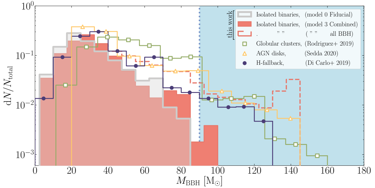
Figure 2.5: M_{\text{BBH}} distribution for BBH systems from different pathways into the PISN mass gap. We compare the distribution of total BBH masses, M_{\text{BBH}} , of multiple generations of BH-mergers in globular clusters (green open squares, Rodriguez et al., 2019a ), multiple generations of BH-mergers in AGN disks (yellow open triangles, Sedda, 2020 ) and stellar mergers in young stellar clusters assuming full H-fallback during BH formation (closed dark blue circles, Di Carlo et al., 2019 ) to the effect of super-Eddington accretion in isolated binaries as discussed in this work. The grey line displays the merging population of BBH systems from our Fiducial model (model 0) The dashed and filled orange distributions respectively show the total and merging population of BBH systems from our most optimistic model variation (model 3 combined). The light blue region bordered by dotted lines indicates the approximate location of the PISN gap assuming BHs of equal mass. All distributions are normalized to their respective population of merging BBHs. This is therefore not a prediction for the number of PISN mass gap events.
