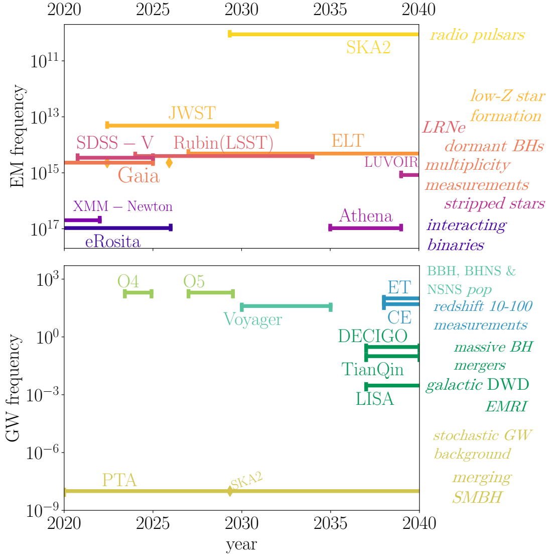
Figure 6.1: A sample of the observational landscape in the next two decades in both EM (top) and GW (bottom) frequencies. Examples of relevant observational constraints that follow from each observing mission are annotated on the right hand side of the plot. Each missions is indicated at either the center of its frequency band, or at the frequency of maximum sensitivity, though some have been slightly shifted for clarity purposes. Diamond symbols indicate either a data release or upgrade to the facility. The dates for third generation GW-missions (2030 and beyond) are very rough estimates. See the text for references and an explanation of the acronyms.
