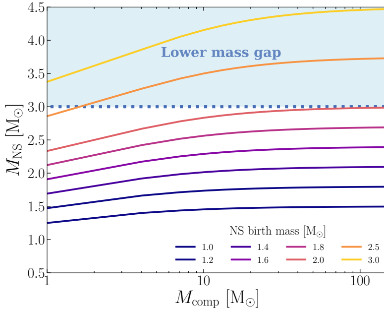
Figure 2.8: The maximum mass for an accreting NS according to Equation 2.2 as a function of the companion mass at the moment of Roche-lobe overflow. This illustrates that only neutron stars that are born close to the lower mass gap will be able to accrete enough to end with a final mass in the lower mass gap.
