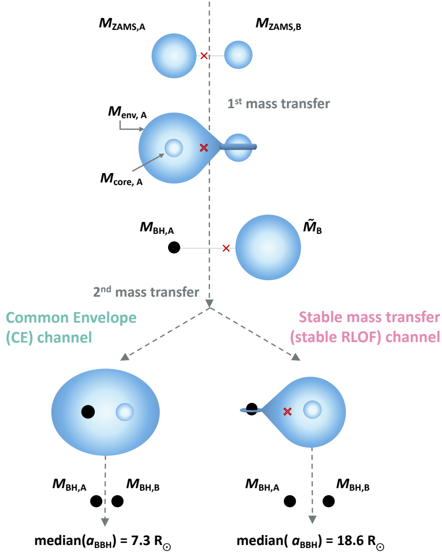
Figure 1.3: Isolated binary channels can broadly be separated based on the stability of mass transfer. Systems that experience only stable mass transfer are part of the ‘stable mass transfer channel’, or stable RLOF channel. Systems that experience unstable mass transfer and a following common envelope (CE) phase are considered part of the ‘common envelope channel’. Figure adapted from van Son et al. (2022b)
