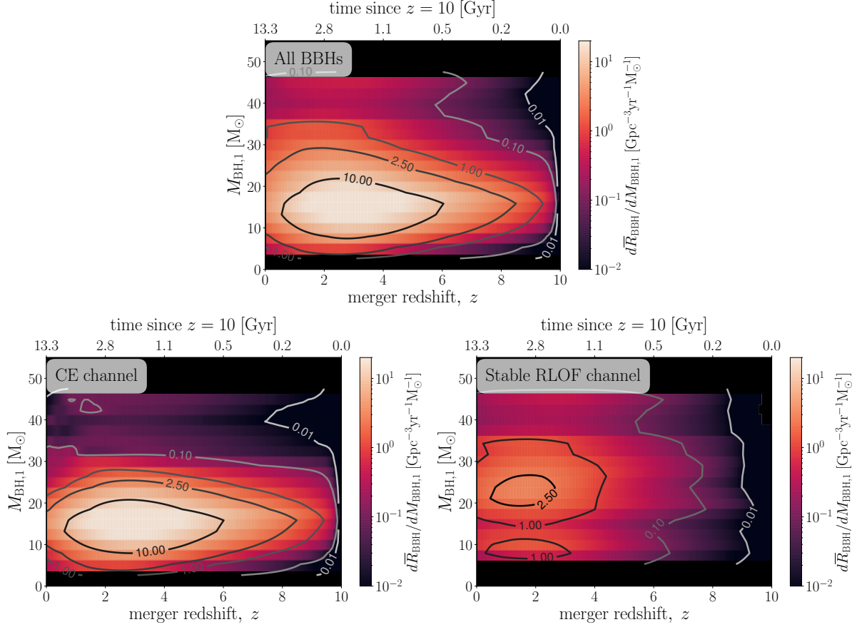
Figure 3.3: The averaged intrinsic merger rate density \bar{R}_{\text{BBH}}(z) , for redshift bins of dz = 0.2 , and primary BH mass bins of dM_{\text{BH},1} = 2.5 M_{\odot} . The top axis shows the time passed since z = 10 , which we have chosen as the redshift of first star formation. The top panel shows the full distribution. The bottom left panel shows mergers of systems that have experienced at least one CE during their evolution, while the bottom right shows mergers of systems that formed through the stable RLOF channel. All panels show a dearth of high mass BHs ( M_{\text{BH},1} \gtrsim 30 M_{\odot} ) merging at higher redshifts ( z > 6 ).
