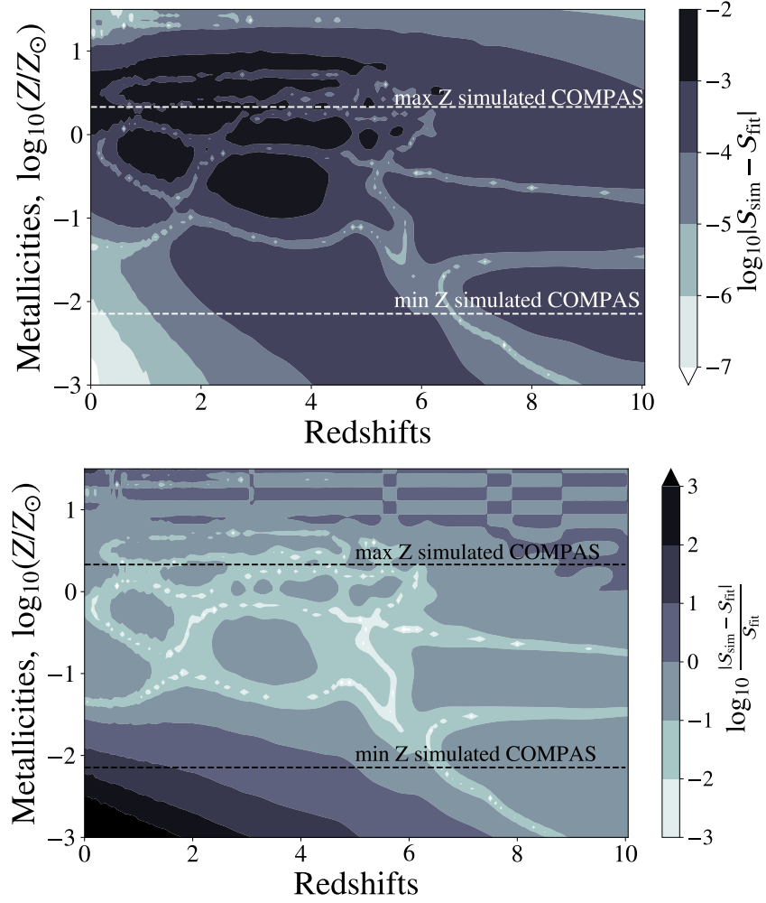
Figure 4.5: log of the residuals (top), and log of the relative error (bottom) between the TNG100 data and our best-fitting model. We show the minimum and maximum metallicity used in COMPAS simulations with dashed lines in each plot.
