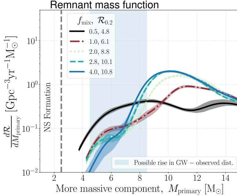
Figure 5.4: Mass distributions in M_{\text{primary}} for BBH and BHNS from the stable channel. We show variations in the supernova remnant mass function using the prescription from Fryer et al. (2022). Similar to the right column of Fig. 5.3, but using a kernel density distribution. To prevent the kernel to smooth over the cutoff mass in M_{\text{primary}} , we only draw the distribution for M_{\text{primary}} values where the corresponding histogram predicts a rate above 10^{-5} \text{ Gpc}^{-3} \text{ yr}^{-1} \text{ M}_{\odot}^{-1} .
