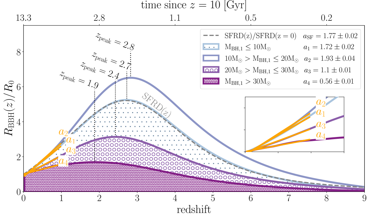
Figure 3.8: Intrinsic BBH merger rate density as a function of redshift, z ( R_{\text{BBH}}(z) , Eq. 3.2), normalized by the rate at redshift zero ( R_0 ), for several bins in primary BH mass. The top axis shows the time since z = 10 , which we have chosen as the redshift of first star formation. The dashed grey line shows the star formation rate density as a function of redshift, \text{SFRD}(z) , normalized by the star formation rate density at redshift 0, \text{SFRD}(z = 0) . The redshift at which the merger rate peaks is annotated with a dotted line for each mass bin. A linear fit to the merger rate density between 0 \leq z \leq 1 is shown with an orange line for each mass bin (these are also highlighted in the inset). The respective slopes of these fits are annotated in the legend. This shows that, at low redshift, the slope of R_{\text{BBH}}(z) is more shallow for higher M_{\text{BH},1} .
