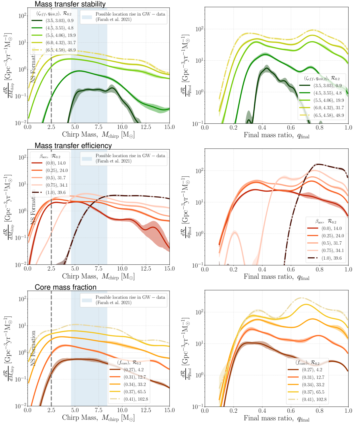
Figure 5.7: The distributions for the chirp mass M_{\text{Chirp}} , and the final mass ratio q_{\text{final}} = M_{\text{secondary}}/M_{\text{primary}} for merging BBH and BHNS. Colours and symbols are the same as the right hand panels of Figure 5.3. This shows that the less massive components can form NS masses, often closing any gap between the most massive NS and the least massive BH.
