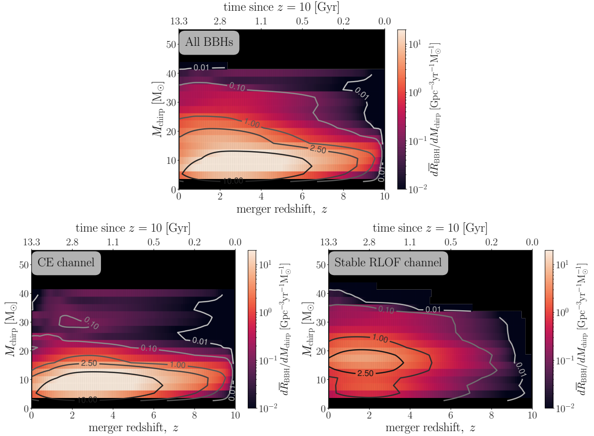
Figure 3.12: The averaged intrinsic merger rate density \bar{R}_{\text{BBH}}(z) , for redshift bins of dz = 0.2 , and chirp mass bins of dM_{\text{chirp}} = 2.5 M_{\odot} . The colours and symbols are the same as in Figure 3.3.
