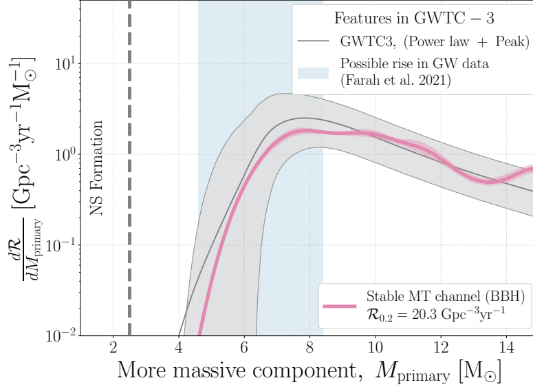
Figure 5.1: Intrinsic distribution of primary masses from BBH merging at redshift 0.2. We show the fiducial predictions for the stable channel in the pink kernel density distributions. The light-shaded area shows the 90% sampling uncertainty as obtained from bootstrapping. The total merger rate of BBHs at z = 0.2 is annotated in the legend. The power law + peak model from Abbott et al. (2021f) is shown in grey, light grey bands show the 90% credible intervals. We indicate a tentative rise observed in the GW data with filled blue (see text). We see that the local rate and the location of the peak at the low mass end of the primary BH mass distribution can be explained remarkably well by the stable channel under our fiducial assumptions.
