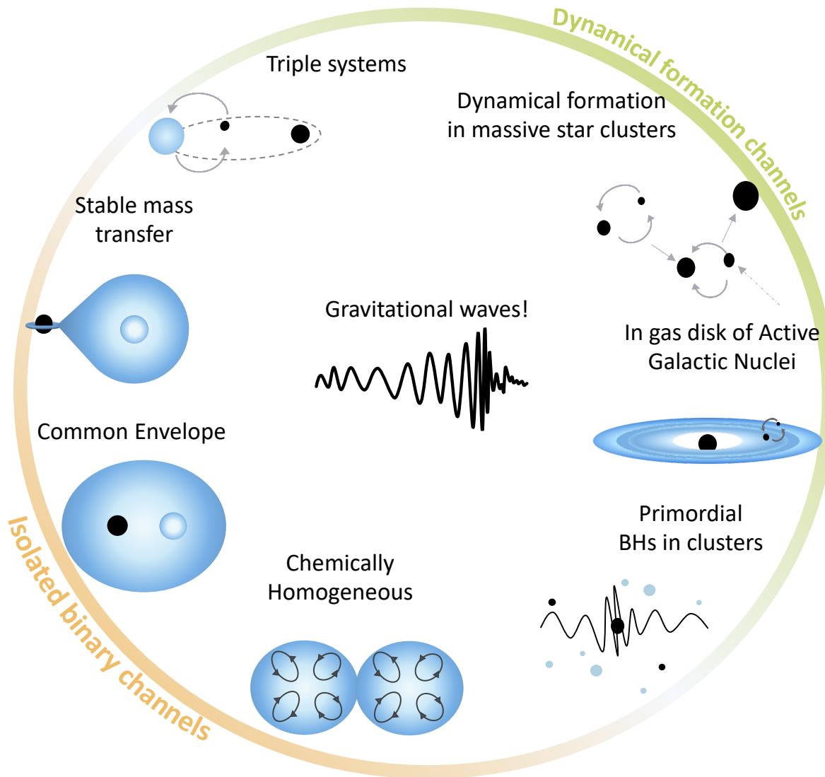
Figure 1.2: Cartoon depictions of the many channels that have been proposed to lead to merging double compact object formation. See text for details.
