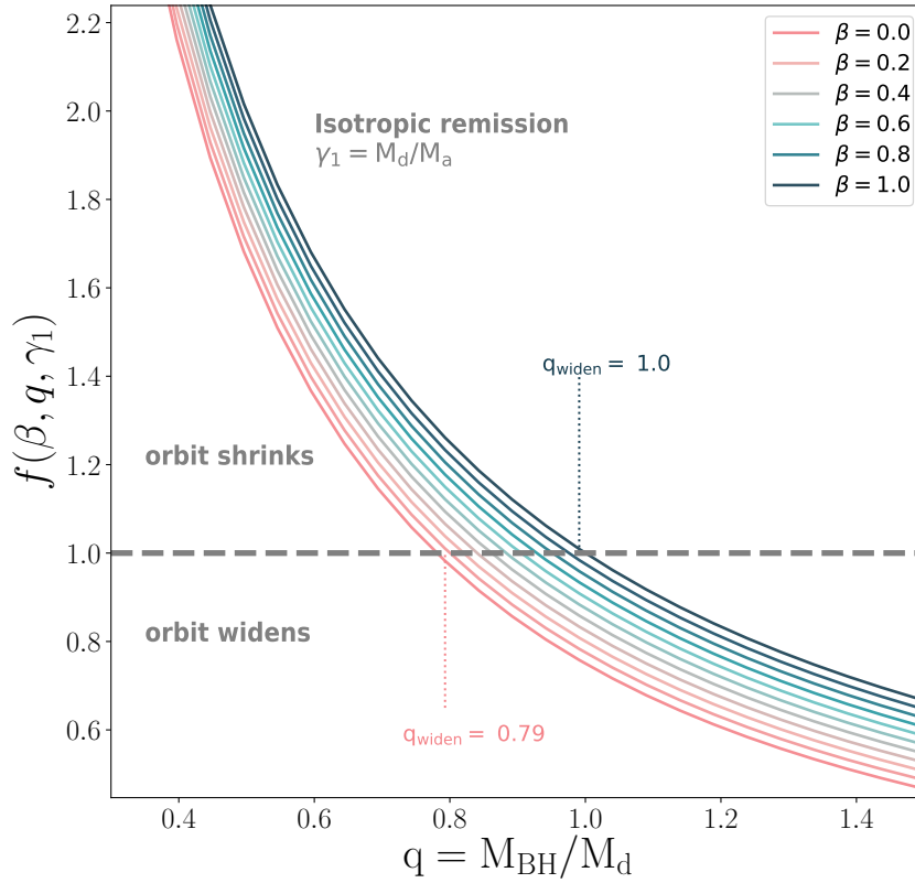
Figure 2.9: Parametrisation of the specific orbital angular momentum evolution that determines whether mass transfer will shrink (above the dashed black line) or widen (below the dashed black line) the binary orbit. The conservativeness parameter \beta varies from completely non-conservative ( \beta = 0 ) to completely conservative ( \beta = 1 ). This assumes isotropic reemission of the ejected matter, i.e., assuming the ejected matter carries the specific angular momentum of the accretor.
