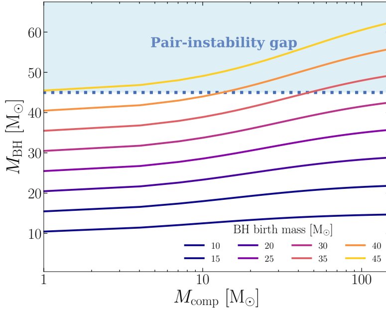
Figure 2.2: The maximum mass for accreting BHs in model variation two, the CE accretion model, following Equation 2.2 as a function of the companion mass at the moment of Roche-lobe overflow. This illustrates that only BHs with a birth mass close to the PISN gap can potentially accrete enough to end with a final mass in the gap.
