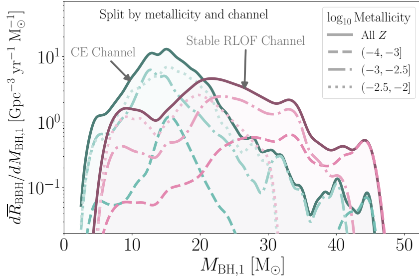
Figure 3.13: Distribution of primary BH masses M_{\text{BH},1} split by formation channel and birth metallicity, for merger redshifts between 0 \leq z < 0.5 .
