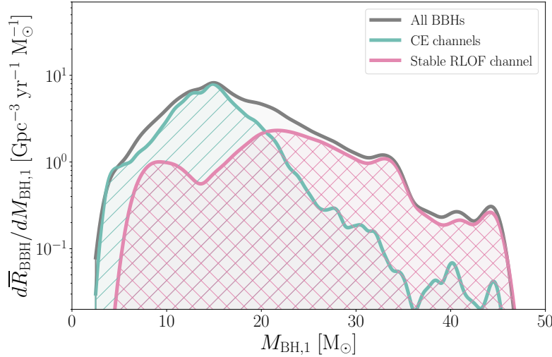
Figure 3.5: Distribution of primary BH masses M_{\text{BH},1} split by formation channel, for merger redshifts between 0 \leq z < 0.5 .
