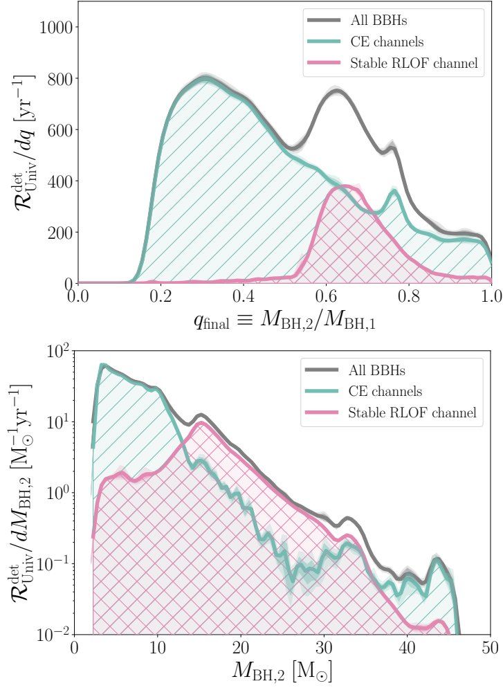
Figure 3.9: Distributions of mass ratios, q_{\text{final}} , and secondary masses, M_{\text{BH},2} , for BBHs seen by a hypothetical perfect detector ( \mathcal{R}_{\text{Univ}}^{\text{det}}(\zeta) , equation 3.6). Each panel shows the distribution for all systems in grey, the stable RLOF channel in cross hatched pink, and the CE channel in line hatched green. The dark and light shaded areas shows the 1- and 2- \sigma sampling uncertainties respectively, obtained through bootstrapping.
